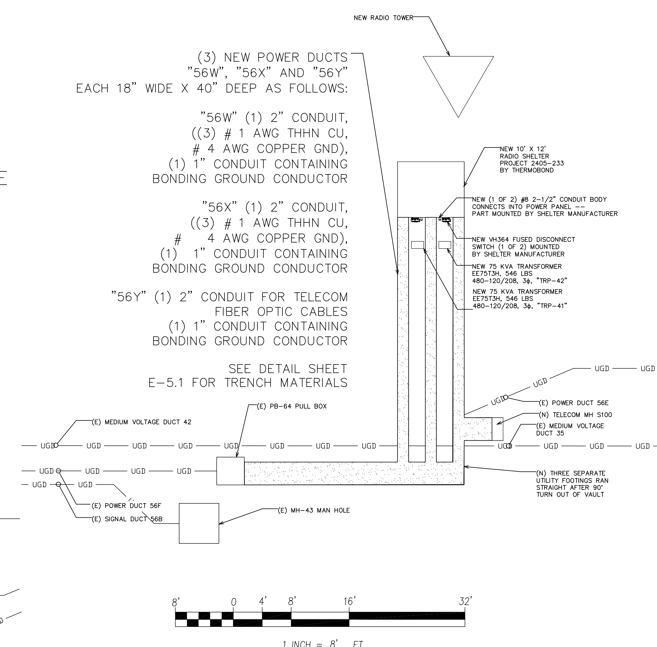
2 RADIO SHELTER PLAN E-3 SCALE: 1" = 8'
